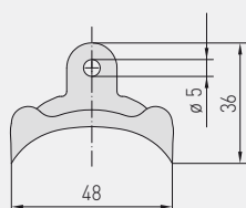
Dimensional drawing MK-05-M
