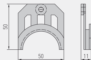
Dimensional drawing MK-05-K
