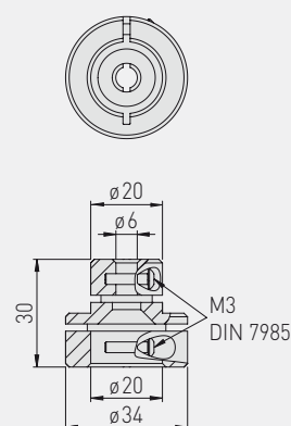
Dimensional drawing TH-ADAPTER-HW
