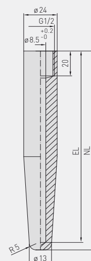
Dimensional drawing ESSH
