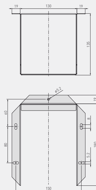
Dimensional drawing
