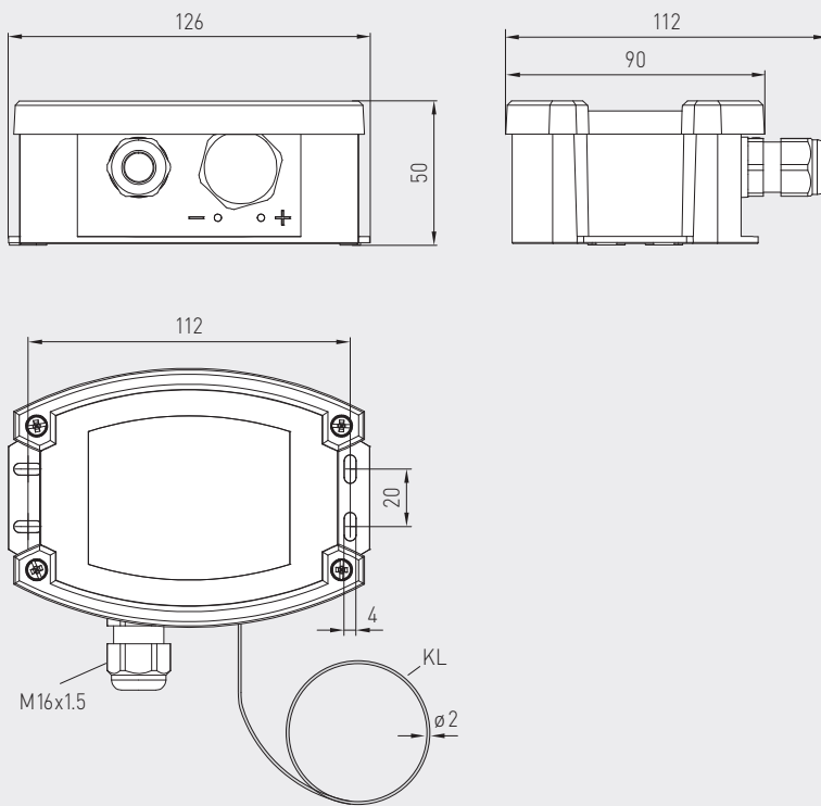
Dimensional drawing
