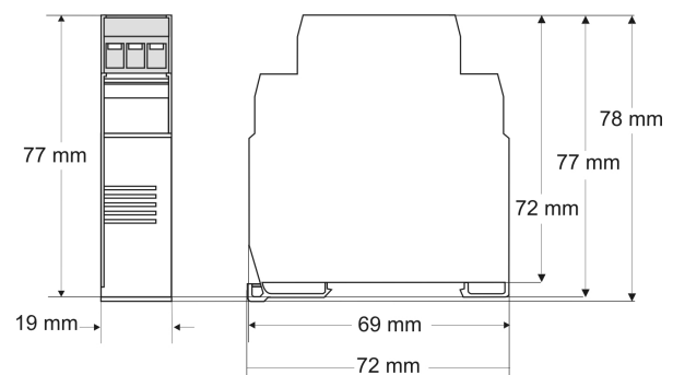
Figure 3 – Dimensions
